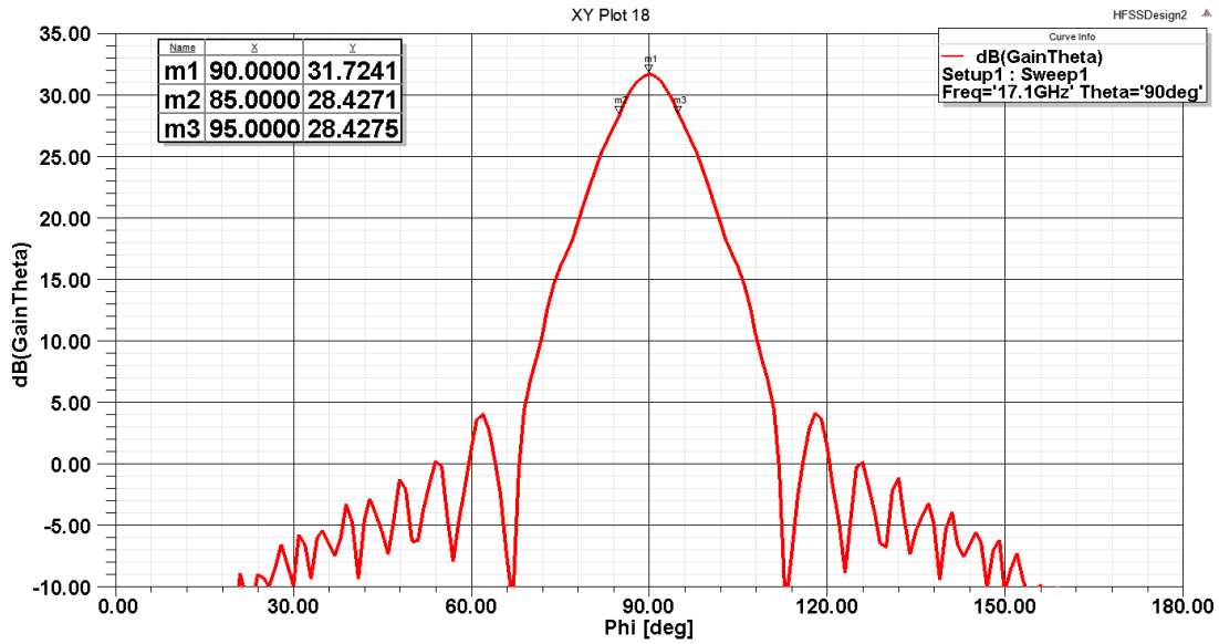
Elevation Pattern
