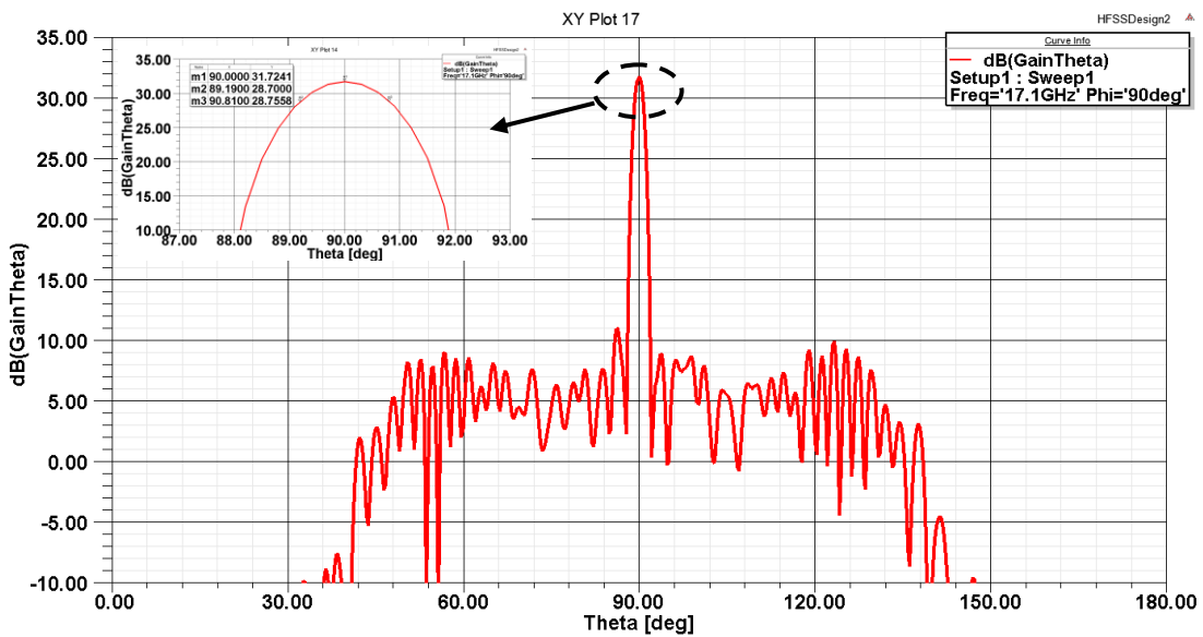
Azimuth Pattern
