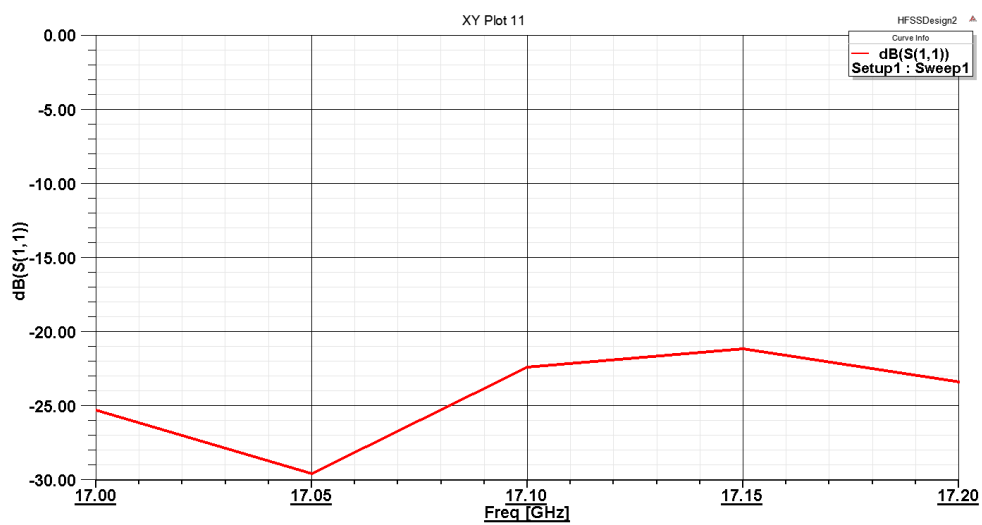
Return Loss
