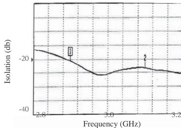
Isolation Between Input Ports
