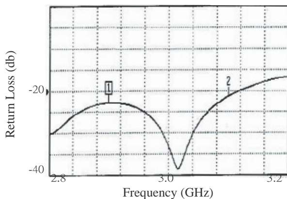
Input Port Return Loss
