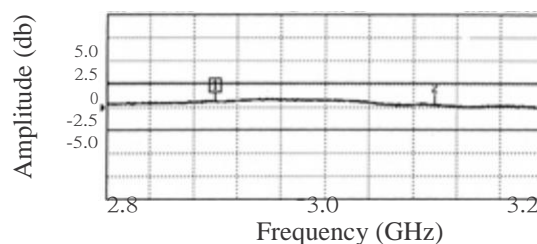
Input Ports Amplitude Balance
