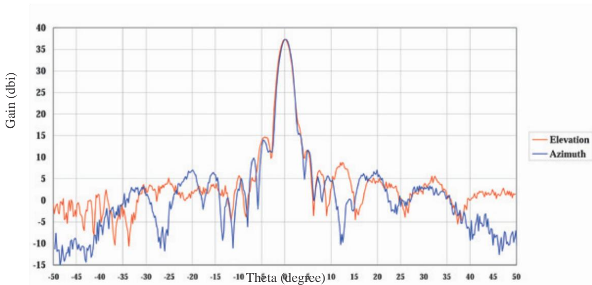
Typical 60cm Reflector Antenna (Model 6389A000) Frequency=18.7 GHz, Gain=37.3 dbi
