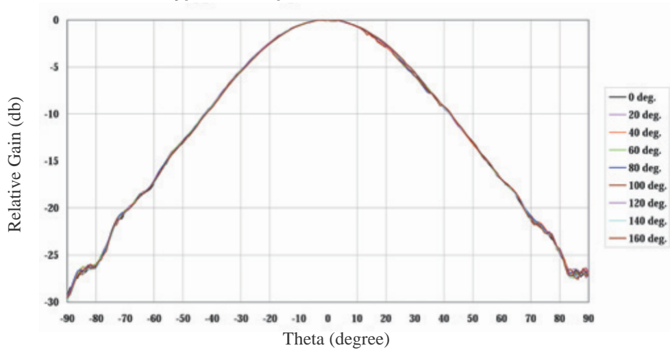
Typical horn patterns with 9 cuts @ 12 GHz
