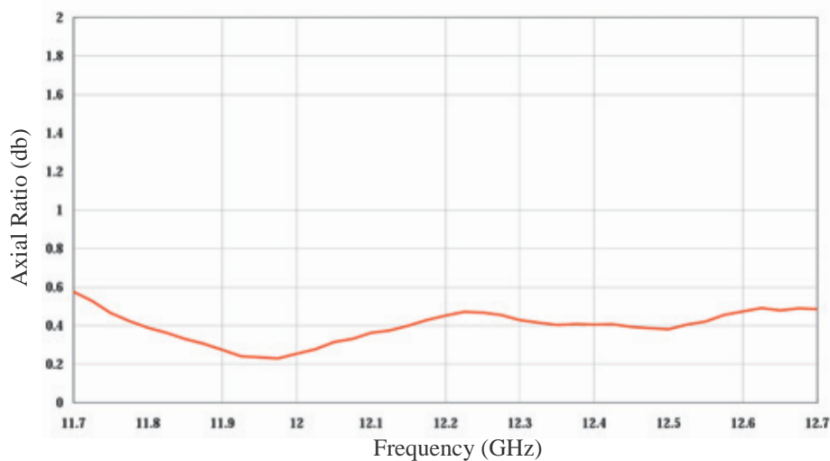
Axial ratio @ theta=0 degree
