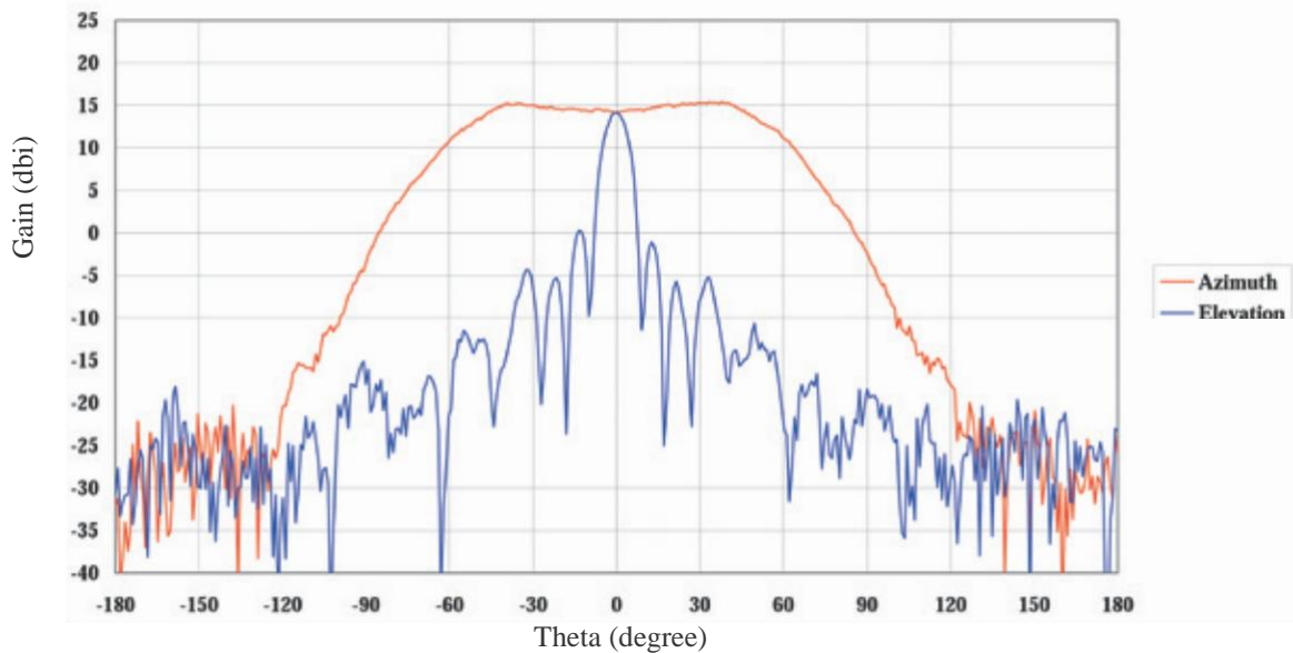
Sector Horn (Model SHA90WR34-V01) V-pol, 90 degree, Frequency=25.5 GHz
