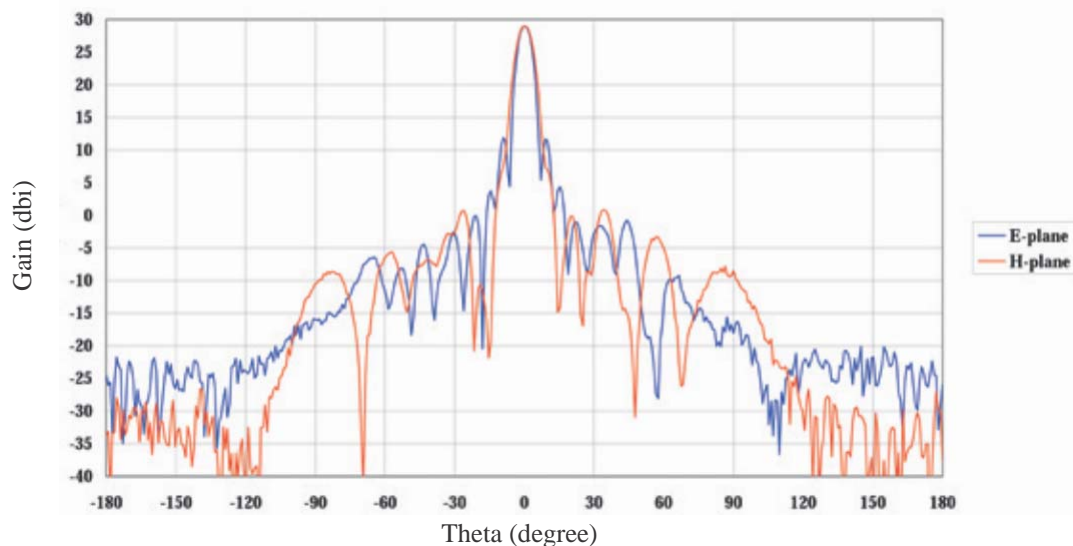
125 mm Lens Horn (Model LHA26WR34-V01) Frequency=25.5 GHz, Gain=29 dbi
